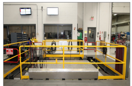
Seismic Testing Platform
