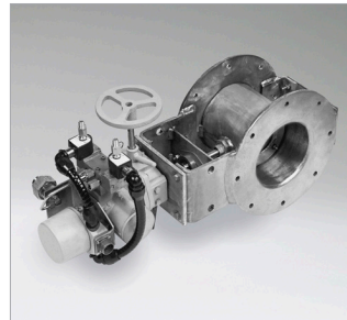
Bubbletight Round Control Damper
