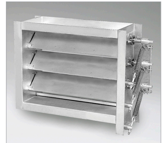
Galvanized Steel Blast Damper
